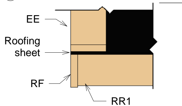
③ Roof Reinforcement
